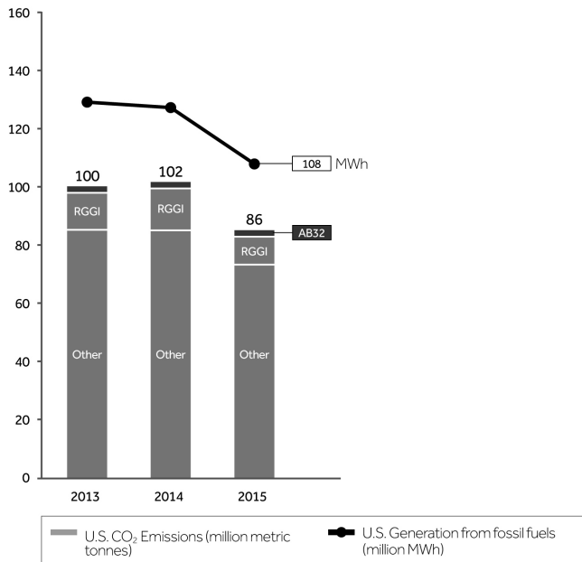
U.S. CO 2 Emissions and Generation
